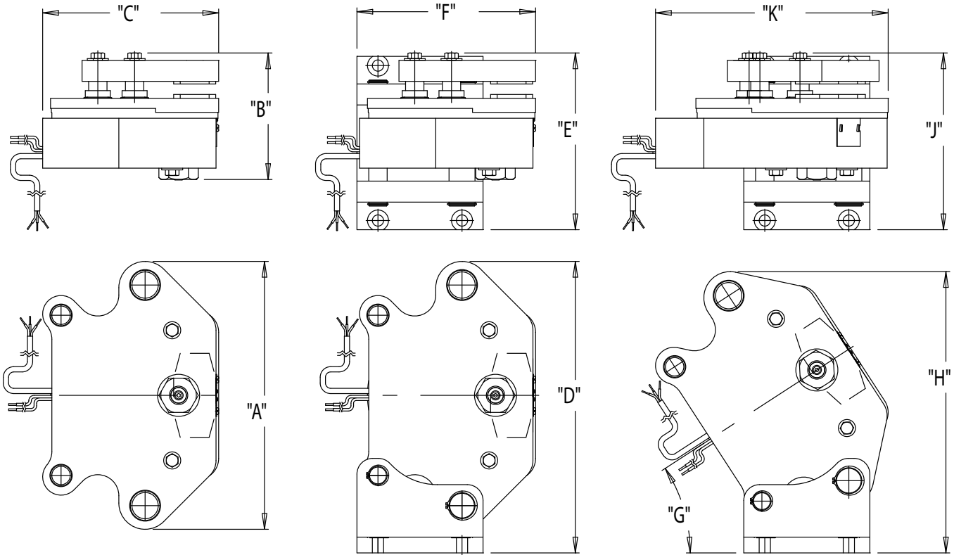
Pin Mounting
